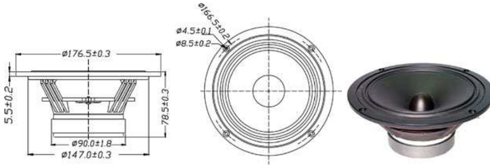
6.5" PPM WOOFER
